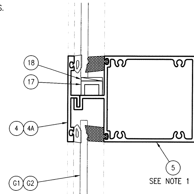
2 VERTICAL CROSS SECTION Shown w/ 1/4" Glass Scale: 6" = 1'-0"
