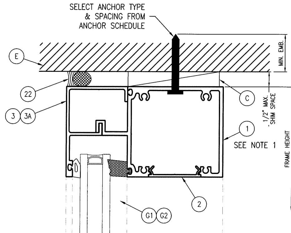
1 VERTICAL CROSS SECTION Shown w/ 1" Glass Scale: 6" = 1'-0"
